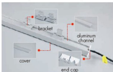
(6) 150° Rotatable Bracket & Aluminum Channel & PC Transparent Cover & End Cap & Screw
