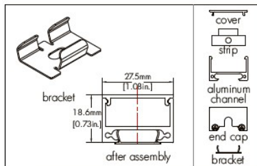
(1) Fix the bracket to the mounting surface by screw. (2) Fix the strip to the aluminum channel by adhesive tape. (3) Fix the cover and the end caps to the aluminum channel by screw. (4) Clip the aluminum to the bracket.
