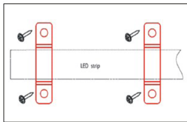
(1) Press the clip against the LED strip.
