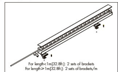
(1) Fix the bracket to the mounting surface by screw. (2) Fix the strip to the aluminum channel by adhesive tape. (3) Fix the cover and the end caps to the aluminum channel by screw. (4) Clip the aluminum to the 150° rotatable bracket.
