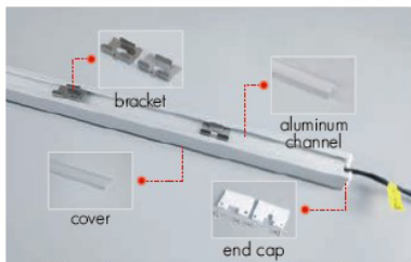
(3) Bracket & Aluminum Channel & Screw Or (4) Bracket & Aluminum Channel & Screw & PC Transparent Cover & End Cap
